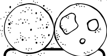
first contact
