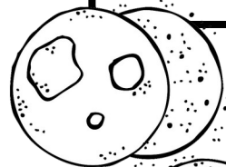
third contact
