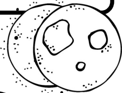
second contact
