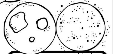
fourth contact
