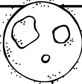
totality
