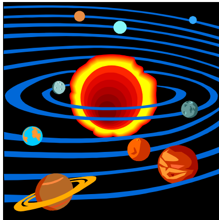
solar system
