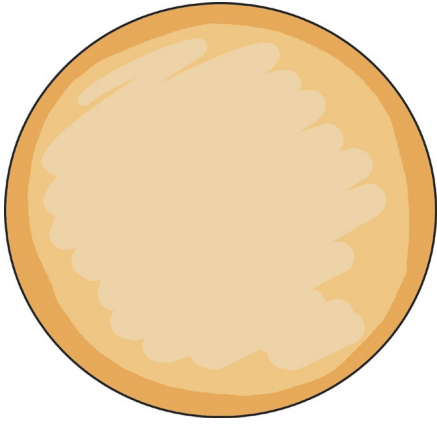
full moon
