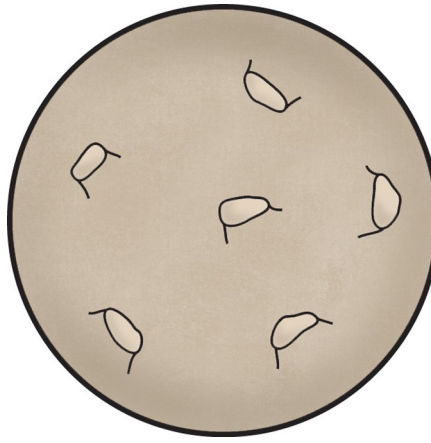
Mercury
