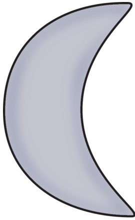
crescent moon
