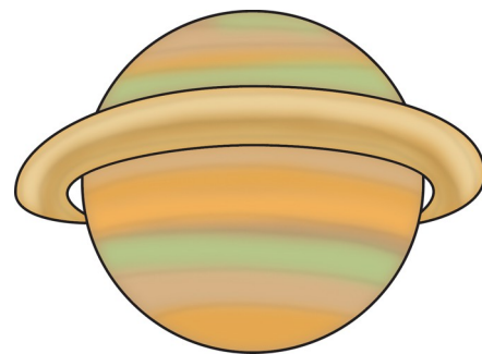
Saturn
