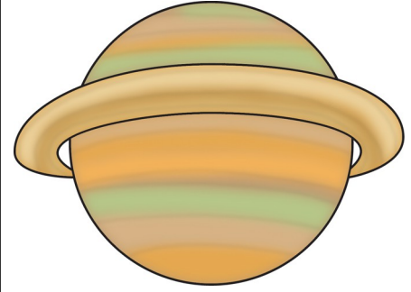
Saturn
