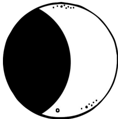
partial eclipse
