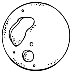
total
