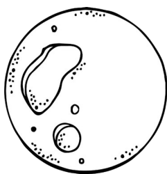
total
